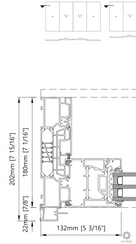
Jamb - Horizontal Two Panel Lift & Slide Door with Fly Screen
