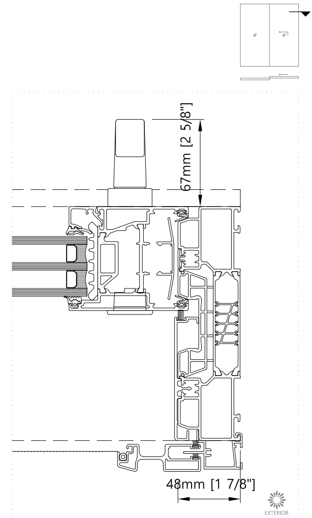
Jamb - Horizontal Two Panel Lift & Slide Door with Fly Screen
