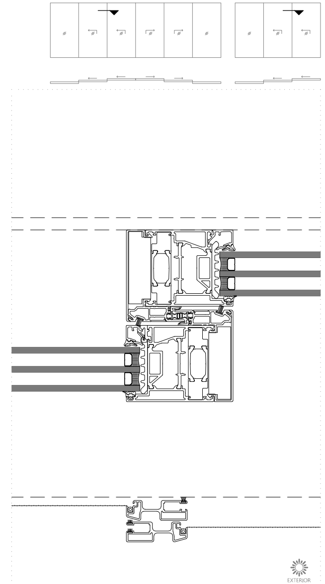
Meeting section - Horizontal Three/Six Panel L&S Door with FS
