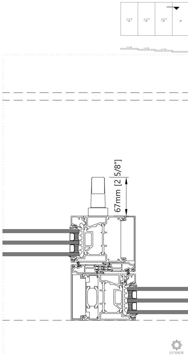
Meeting section - Horizontal Four Panel L&S Door without Fly Screen
