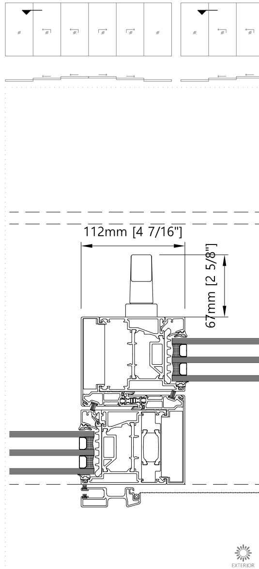
Meeting section - Horizontal Three/Six Panel L&S Door with FS
