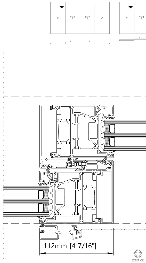
Meeting section - Horizontal Two Panel Lift & Slide Door with Fly Screen
