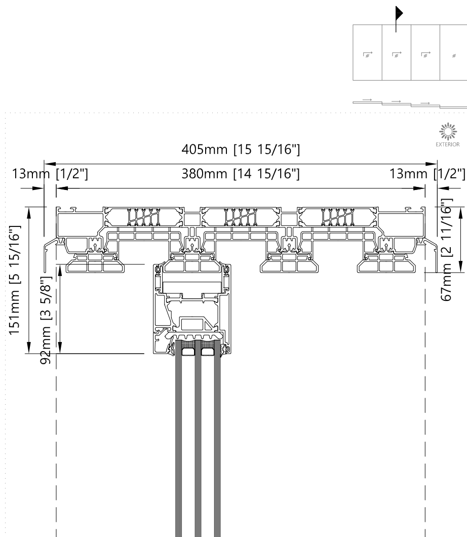
Top - Vertical Four Panel Lift & Slide without Fly Screen
