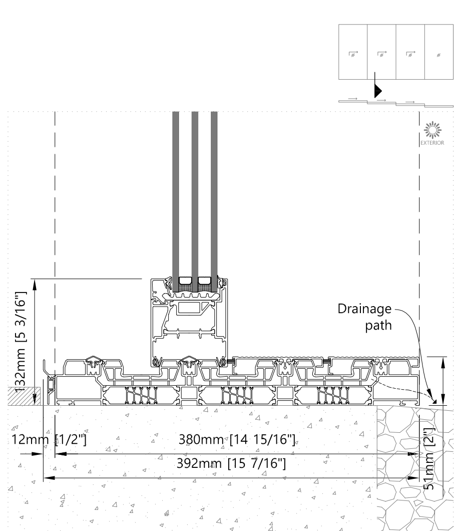
Bottom - Vertical Four Panel Lift & Slide without Fly Screen
