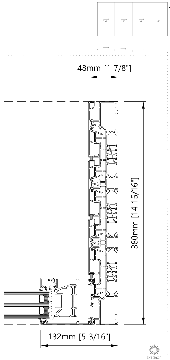
Jamb - Horizontal Four Panel L&S Door without Fly Screen
