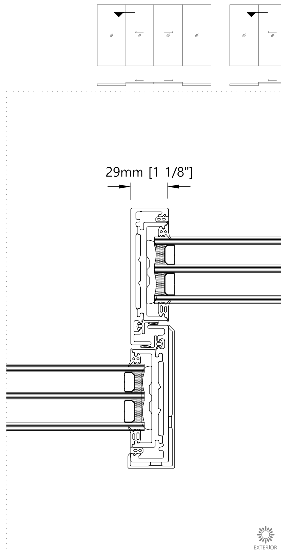
Meeting section - Horizontal Two/Four Panel Sliding Door
