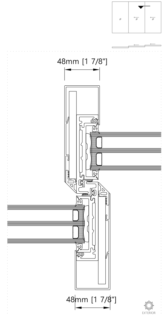
15.2 Meeting section - Horizontal Three Panel Sliding Door with both-side reinforcements
