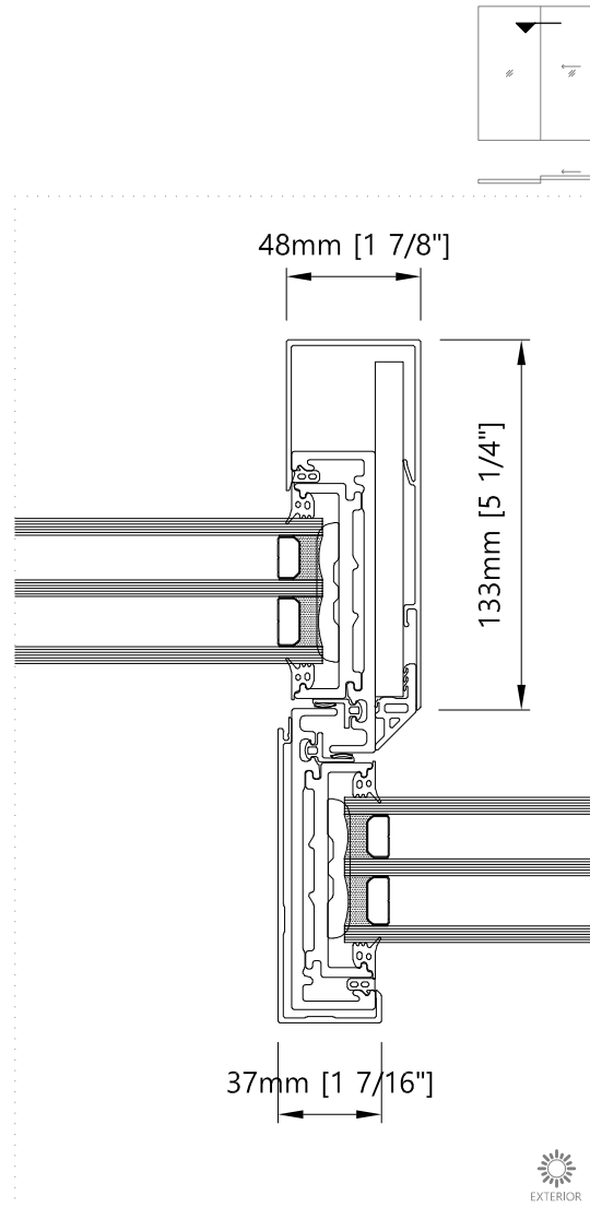
2.2 Meeting section - Horizontal Two Panel Sliding Door with interior reinforcement
