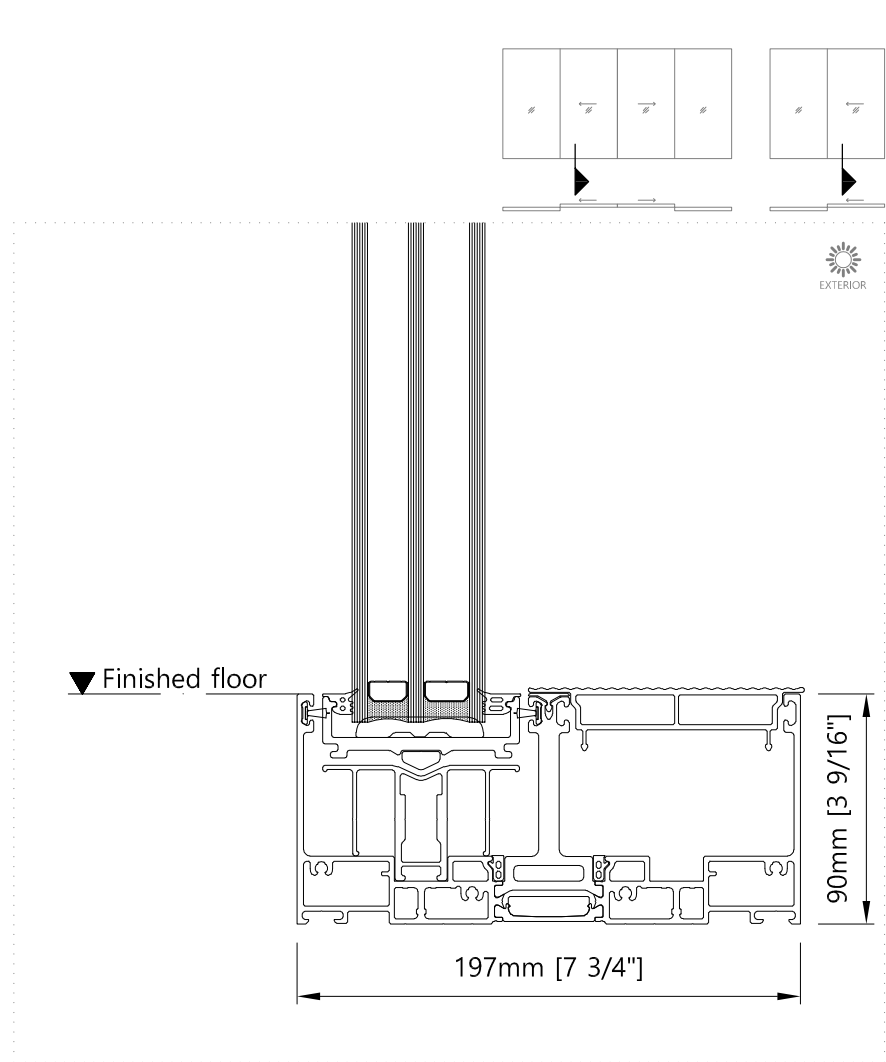
Bottom - Vertical Two/Four Panel Sliding Door
