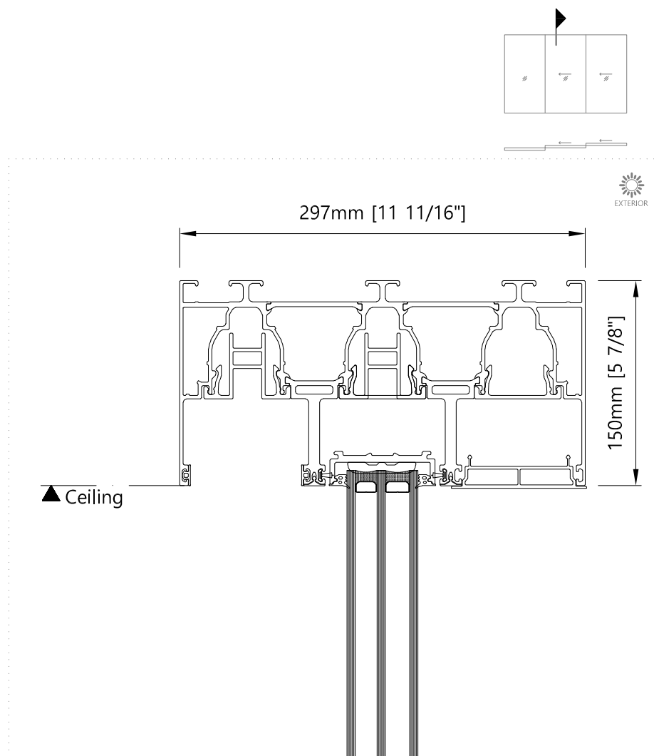
Top - Vertical Three Panel Sliding Door
