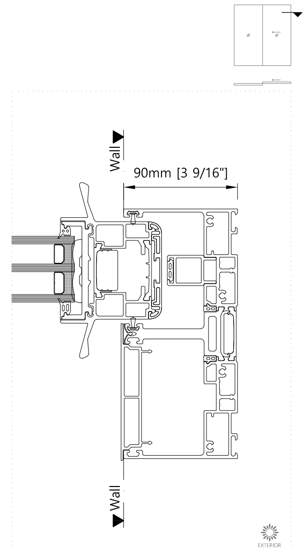
Jamb - Horizontal Two Panel Sliding Door
