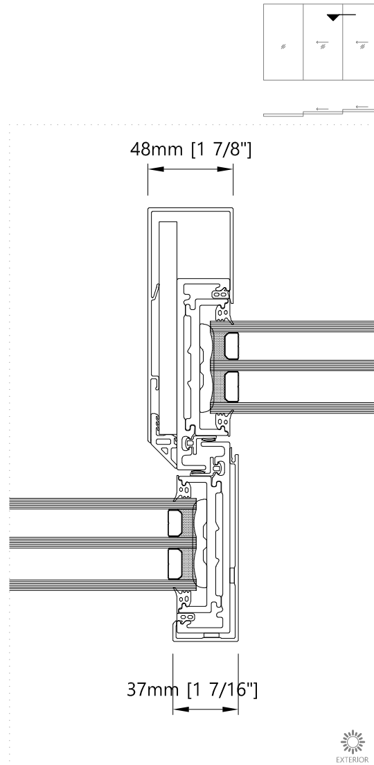
15.1 Meeting section - Horizontal Three Panel Sliding Door with interior reinforcement
