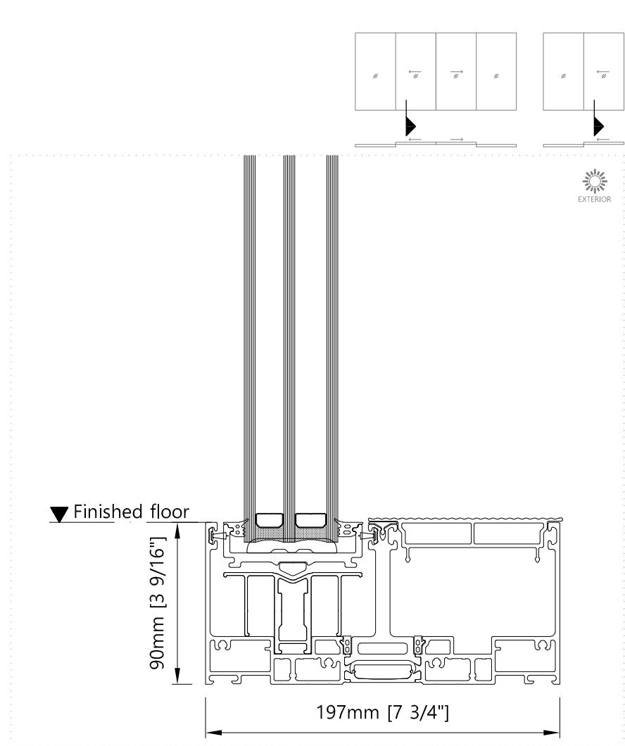
Bottom - Vertical Two/Four Panel Sliding Door
