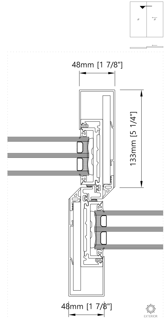
2.3 Meeting section - Horizontal Two Panel Sliding Door with both-side reinforcements
