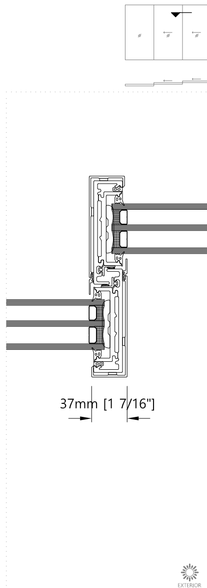
Meeting sec. - Horizontal Three Panel Sliding Door
