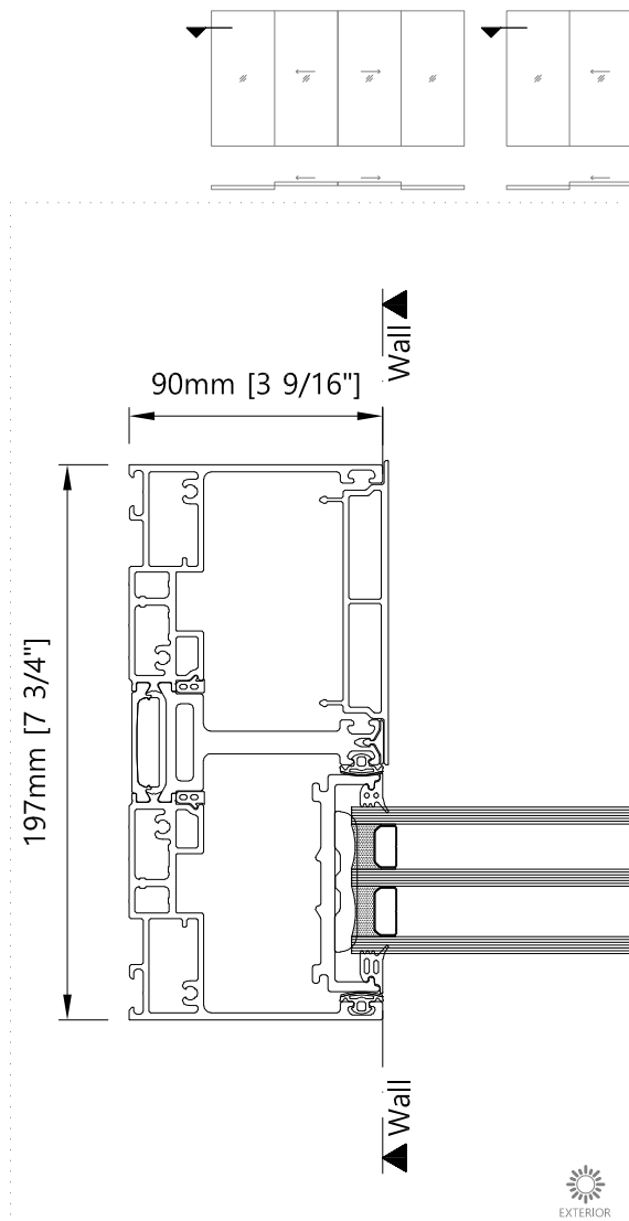
Jamb - Horizontal Two/Four Panel Sliding Door
