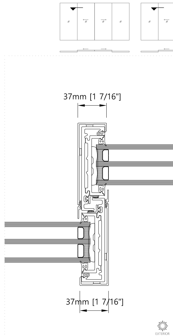
2 Meeting section - Horizontal Two/Four Panel Sliding Door
