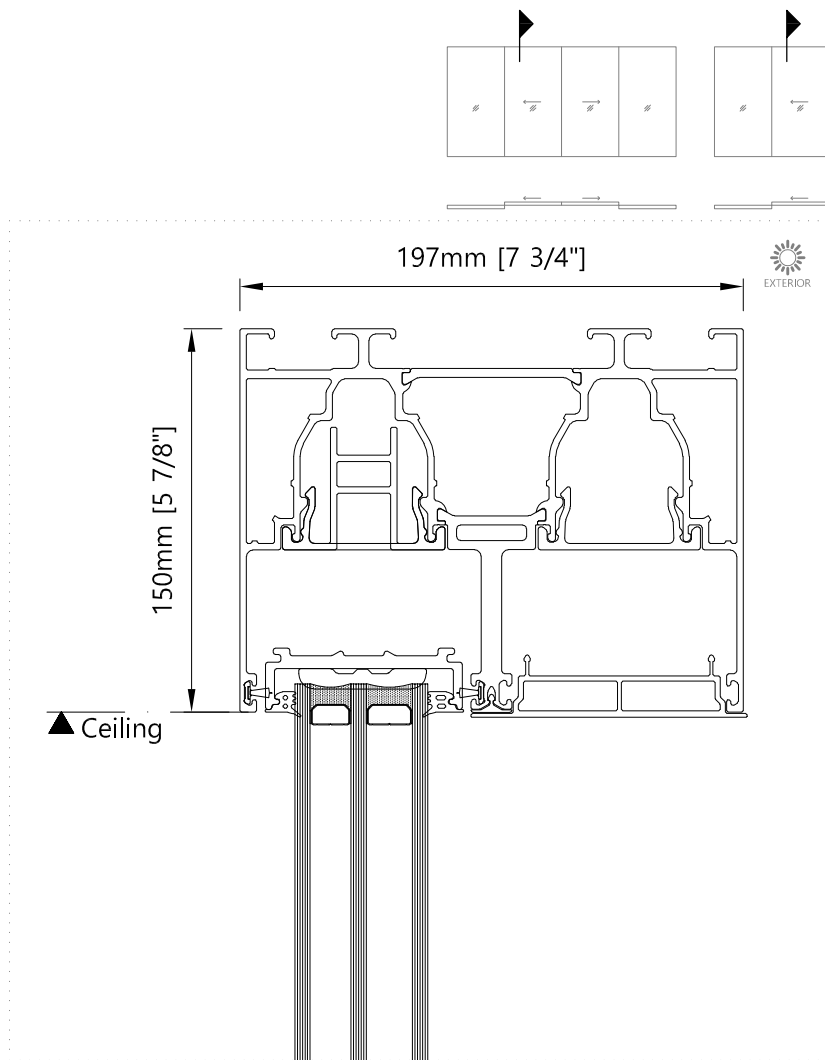
Top - Vertical Two/Four Panel Sliding Door
