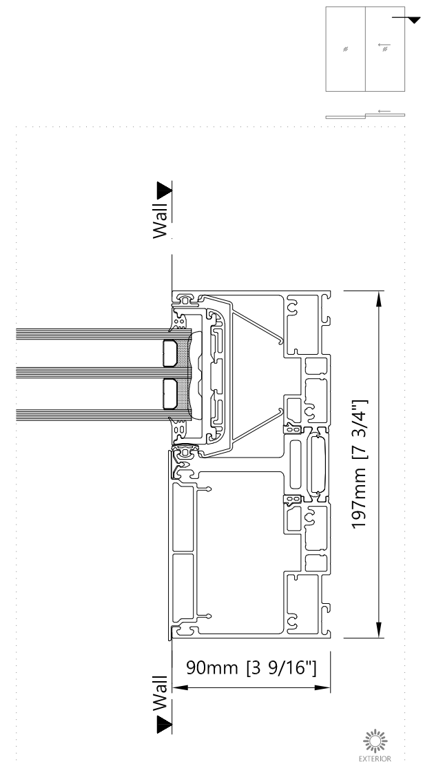
3 Jamb - Horizontal Two Panel Sliding Door
