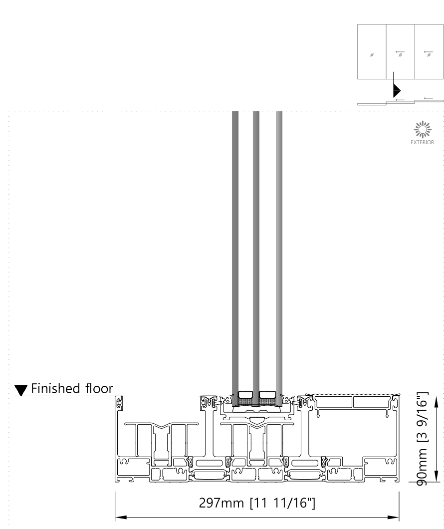
Bottom - Vertical Three Panel Sliding Door
