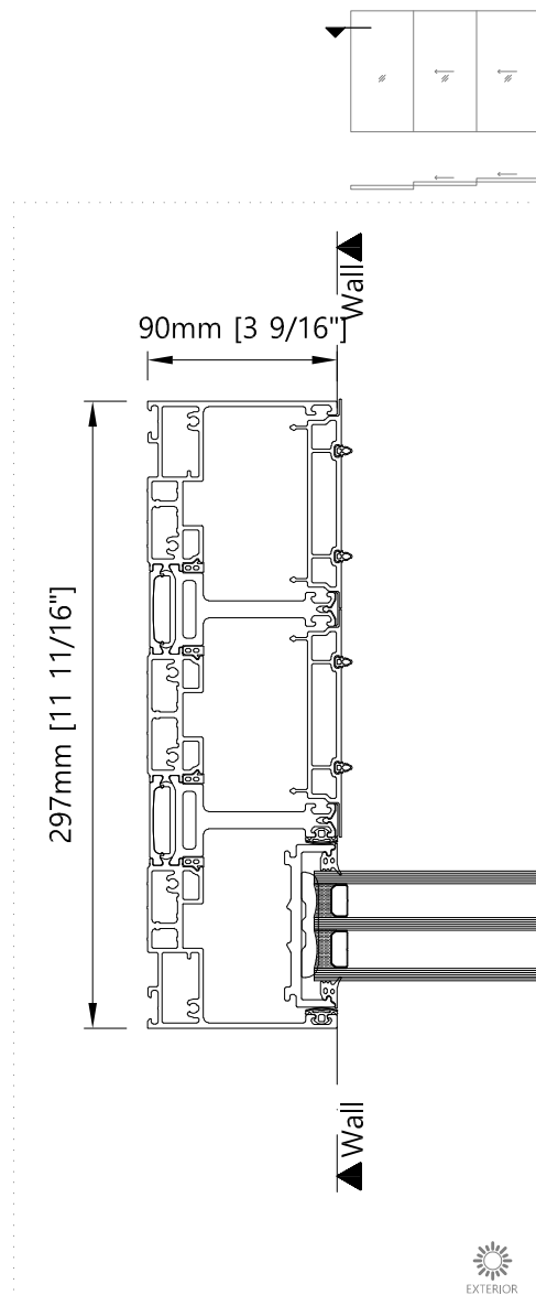
Jamb - Horizontal Three Panel Sliding Door
