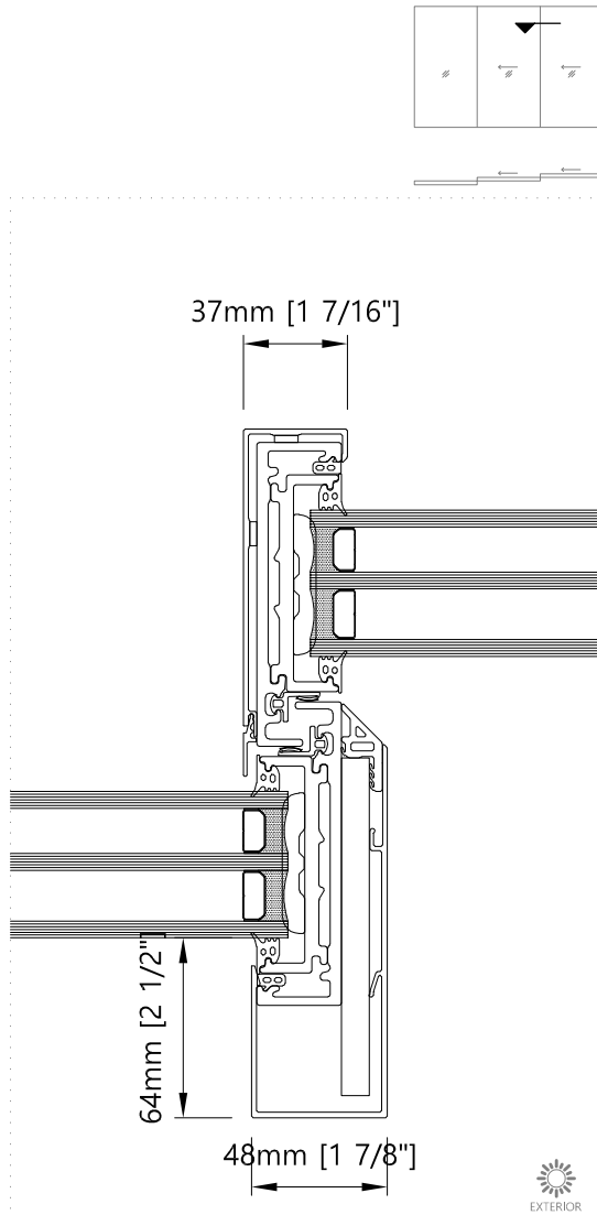
14.1 Meeting section - Horizontal Three Panel Sliding Door with exterior reinforcement
