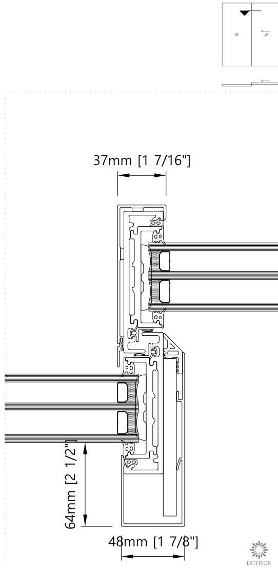
2.1 Meeting section - Horizontal Two Panel Sliding Door with exterior reinforcement
