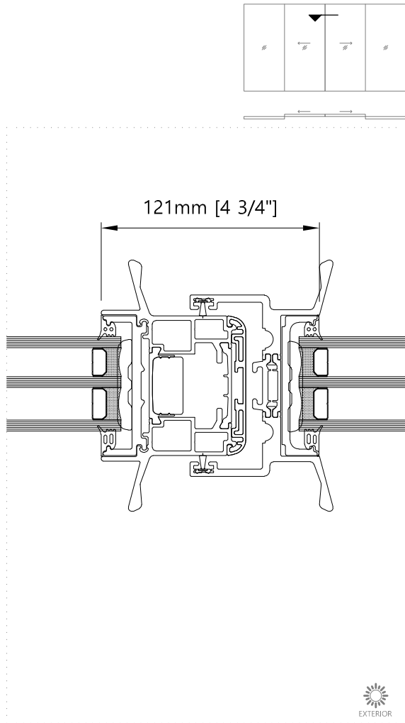
4 Meeting Section - Horizontal Four Panel Sliding Door
